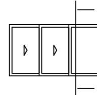
Vertical Section
