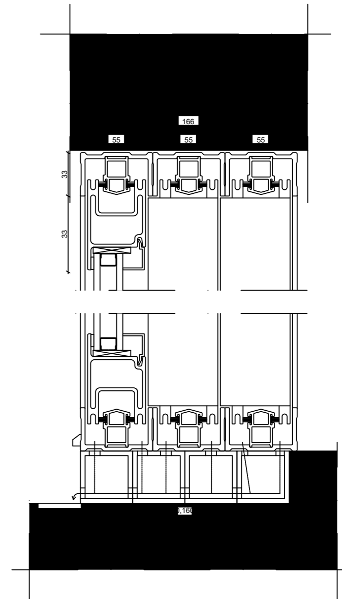
Vertical Section
