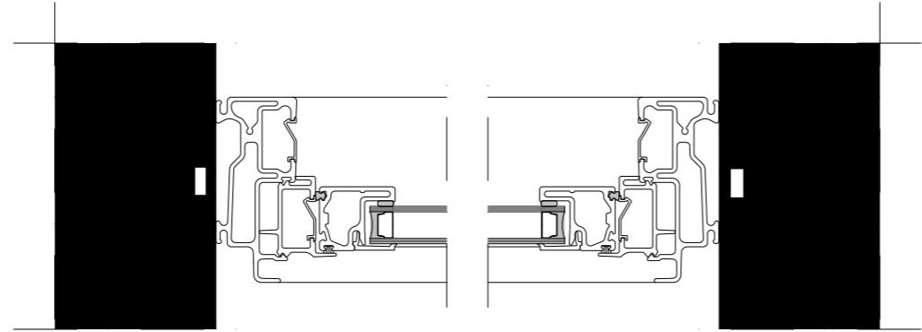
Horizontal Section
